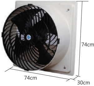
24 inch strong circulation fan
