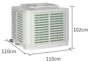
DC environment friendly air conditioner
